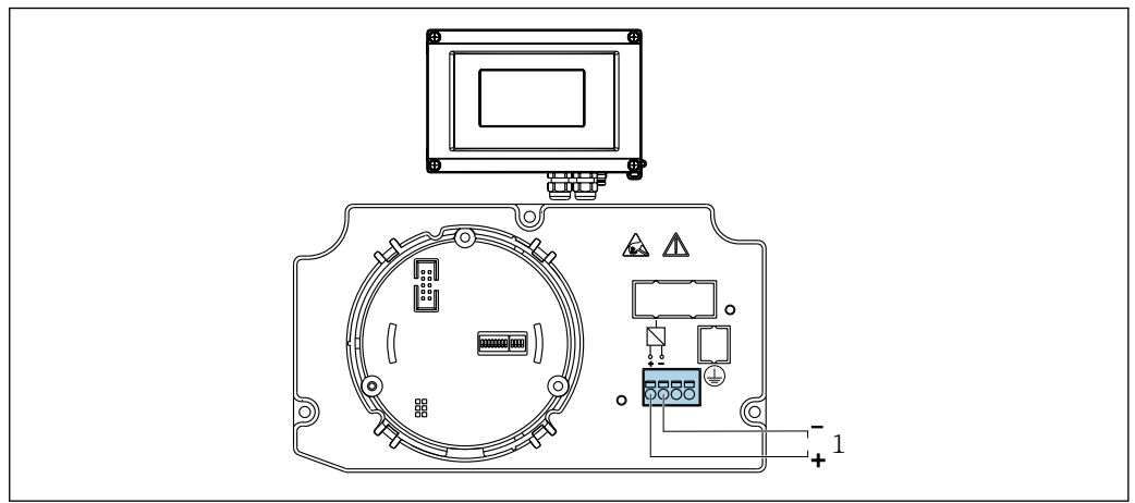
3 Terminal assignment of the field indicator 1 Fieldbus connection
