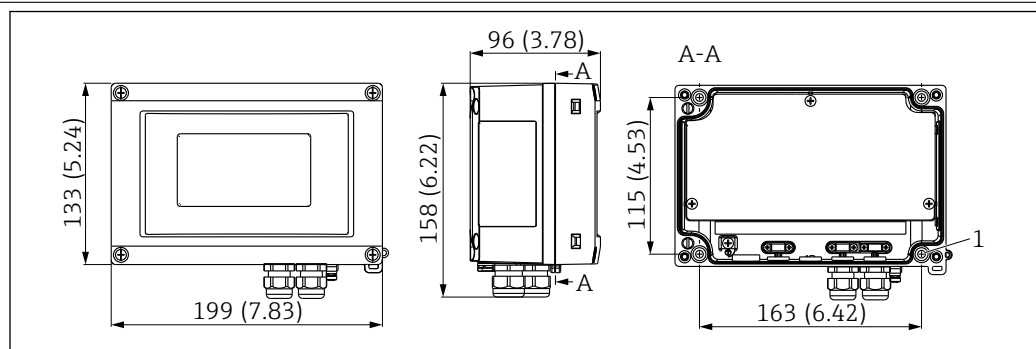
4 Dimensions of the field indicator; dimensions in mm (in)
