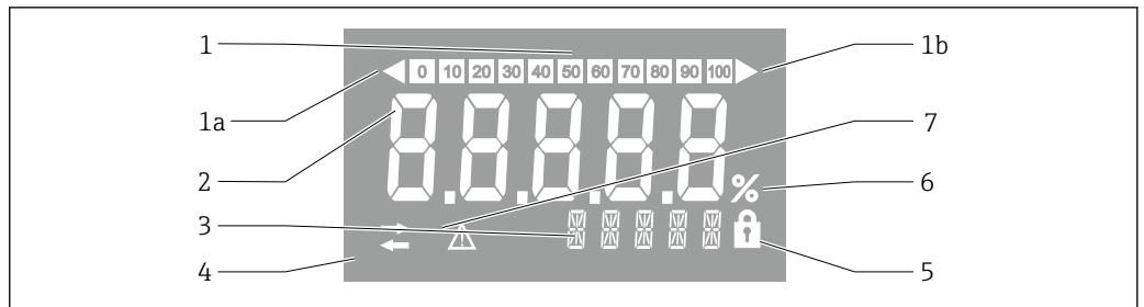
5 LC display of the field indicator (backlit)
