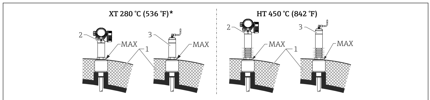
29 Process connection with thread - FMP54, sensor version XT and HT
