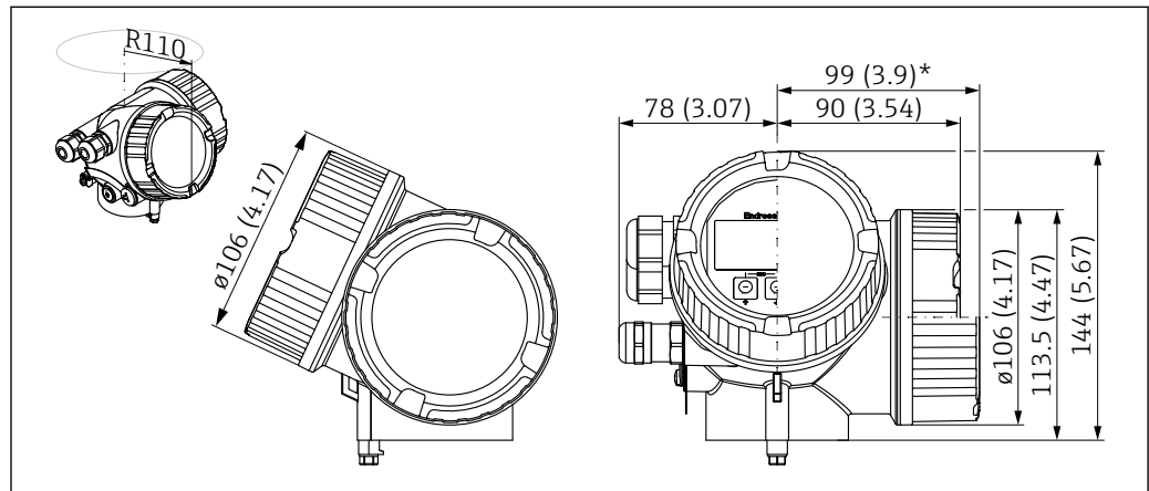
32 Housing GT19 (Plastics PBT); Dimensions in mm (in)
