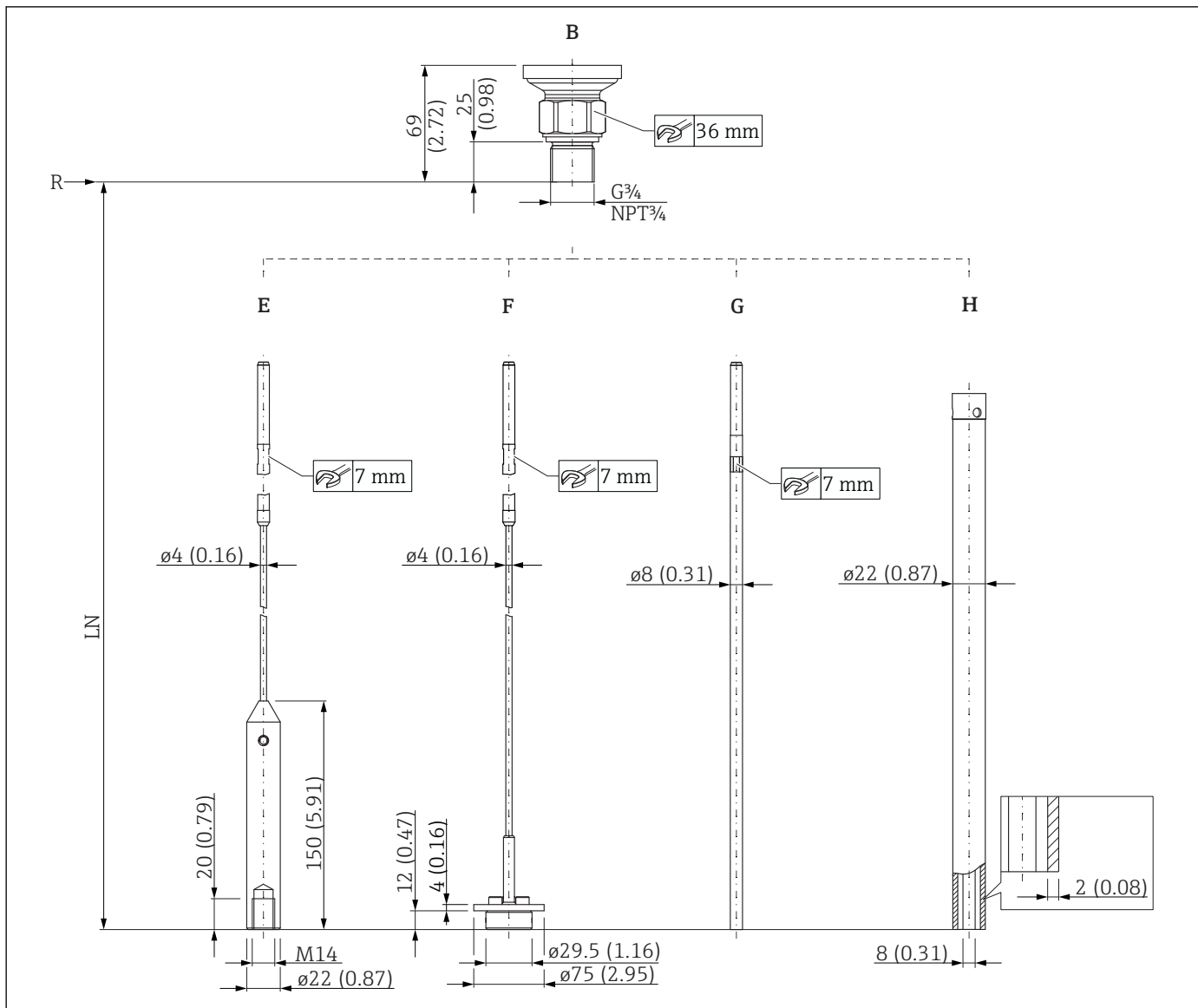
FMP51: Dimensions of process connection (G \frac{3}{4} , NPT \frac{3}{4} ) and probe
