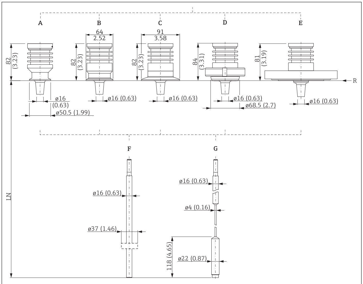
39 FMP52: Process connection / probe. Unit of measurement mm (in)
