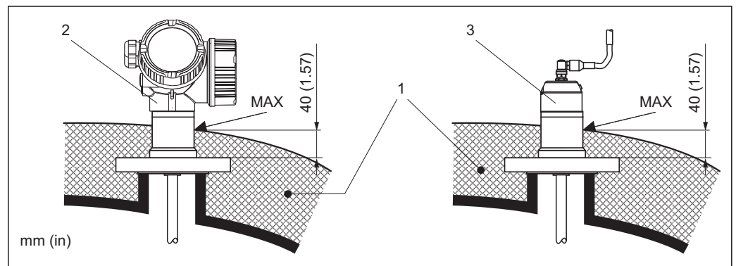
28 Process connection with flange - FMP51, FMP52
