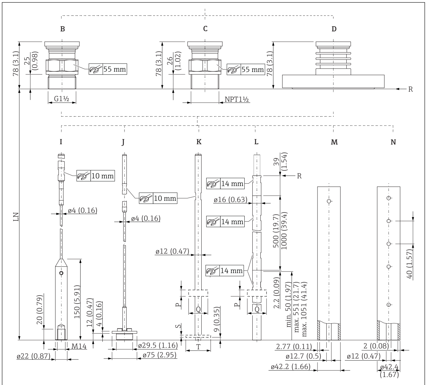
37 FMP51: Process connection / probe. Unit of measurement mm (in)
