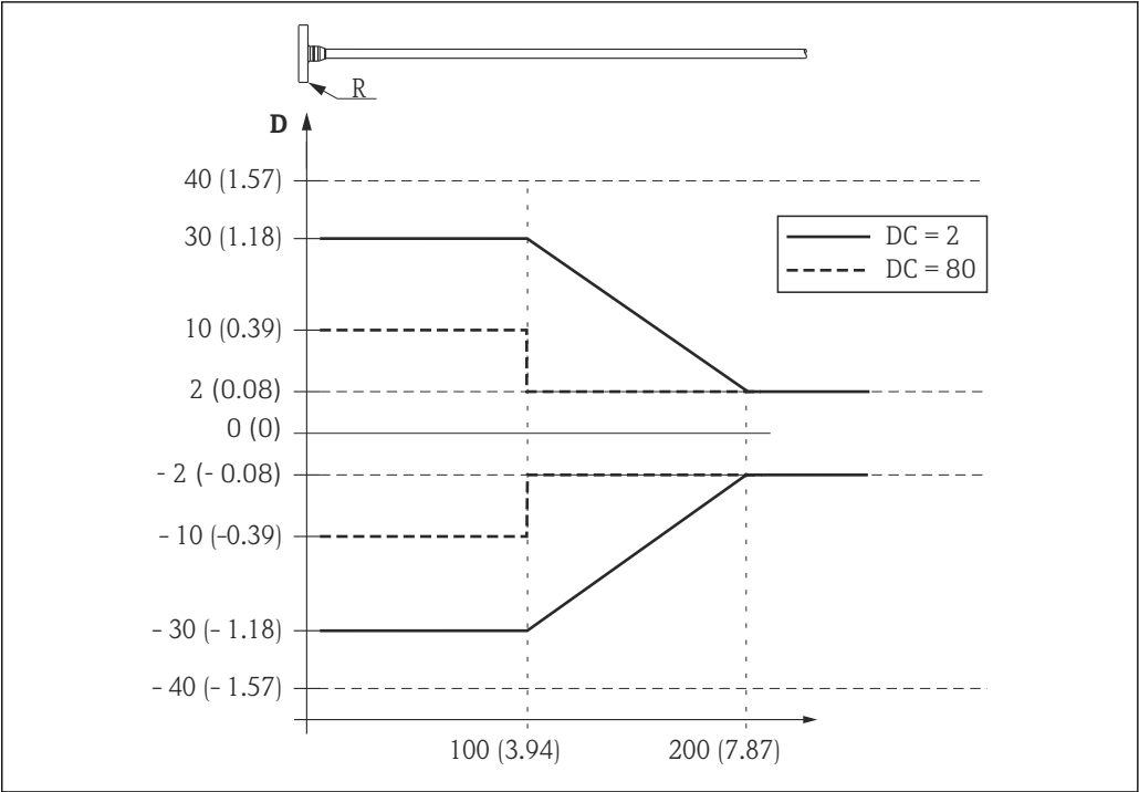
22 Measuring error at the upper end of the probe; dimensions: mm (in)
