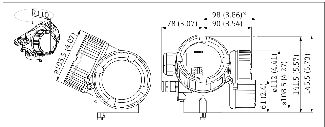
33 Housing GT20 (Alu coated); Dimensions in mm (in)
