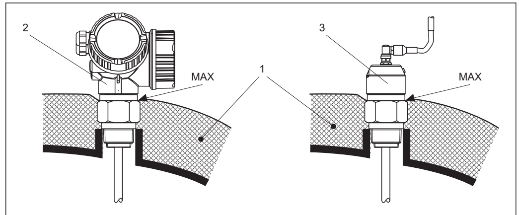
27 Process connection with thread - FMP51
