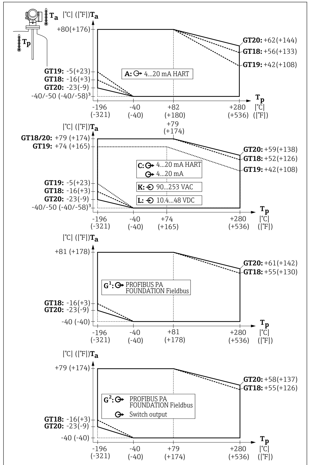
Temperature derating for FMP54 - version XT up to +280 °C (+536 °F)
