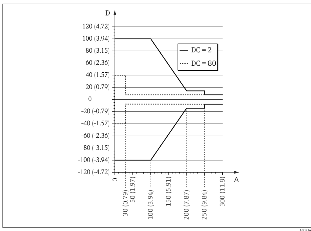
21 Measuring error at the end-of-probe for probes with metallic centering disk (product structure: feature 610 "Accessory mounted", option OA, OB or OC)
