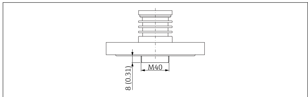
38 Dimensions of AlloyC flanges. Unit of measurement mm (in)
