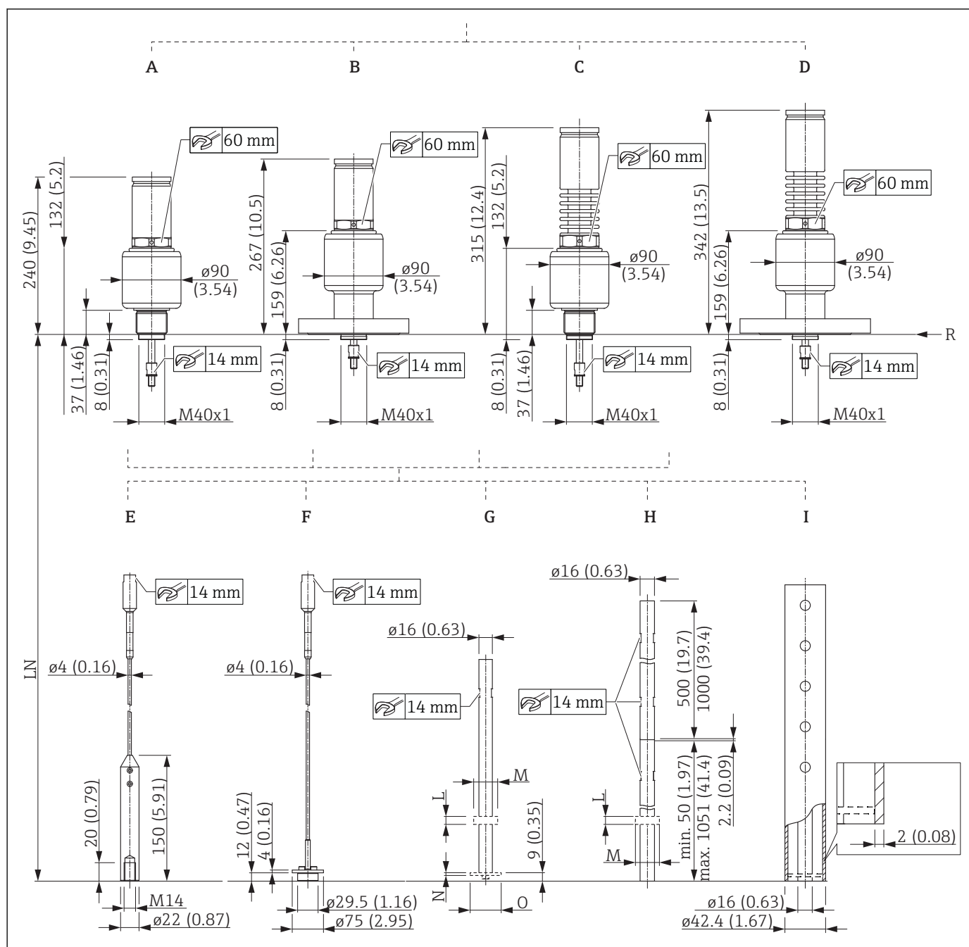
FMP54: Dimensions of process connection and probe
