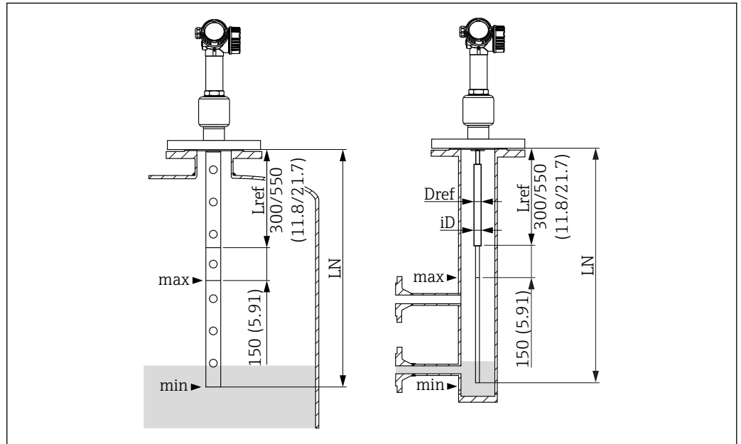
23 FMP54 with reference signal for gas phase compensation; dimensions: mm (in)
