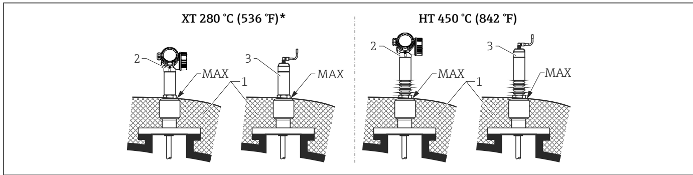
30 Process connection with flange - FMP54, sensor version XT and HT
